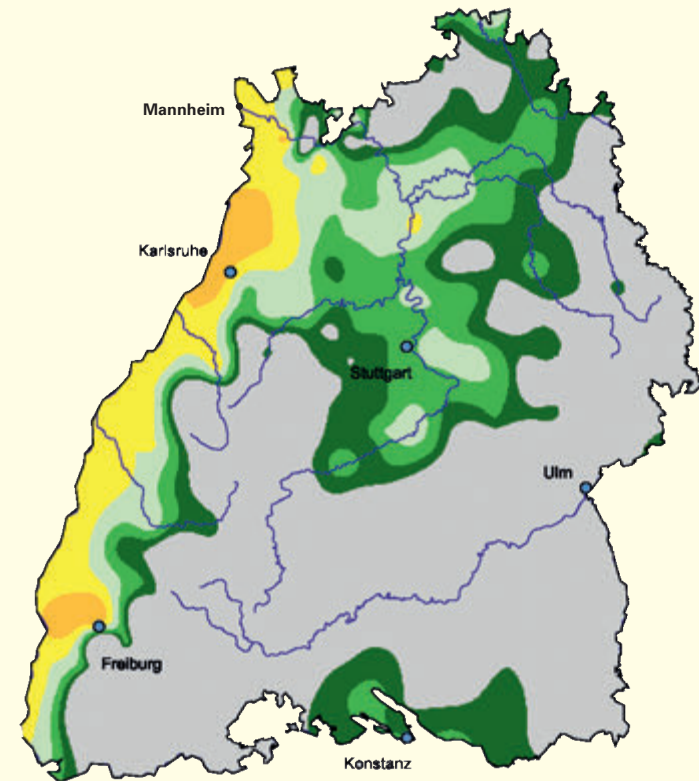
Huglin-Index
